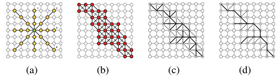
Fig. 4. Chang's Profile recognition and Polygon breaking Algorithm (PPA) (a) Profile recognition (b) Target Connection (c) Polygon breaking (d) Branch reduction
